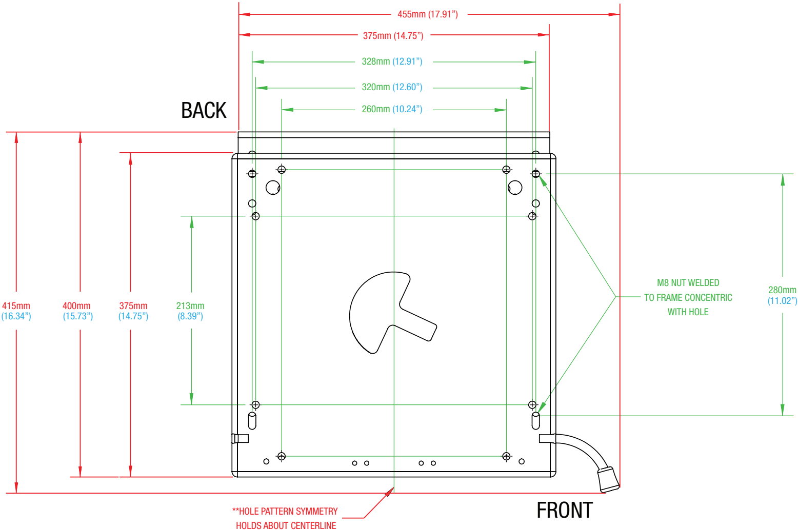
Top Mounting Pattern
